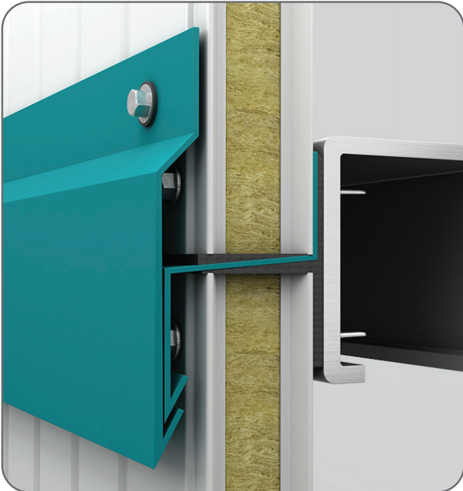
Cephe Panel Ek Detay / Facade Panel Supplementary Detail
