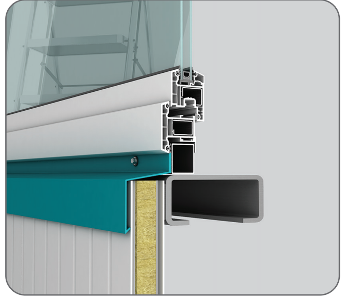
Pencere Alt Detay / Window Lower Detail
