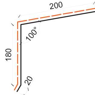
Oluk Etek Profili / Gutter Eave Profile
