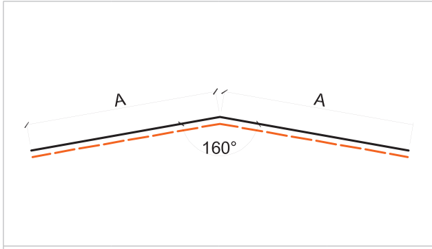
Alt Mahya Profili / Internal Ridge Profile
