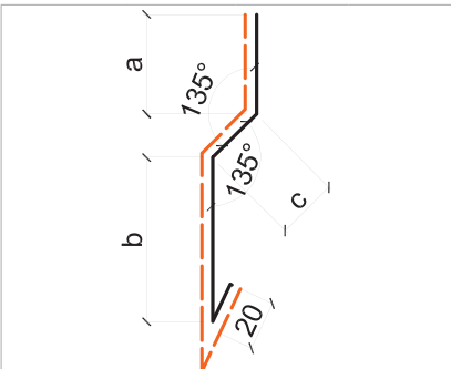
Vida Kapama Profili / Screw Closing Profile
